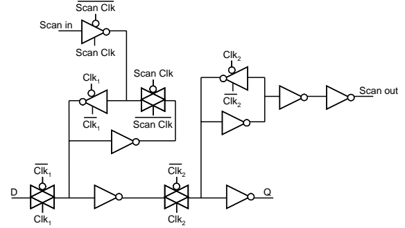
FIGURE 4. Master-Slave Flip-Flop
