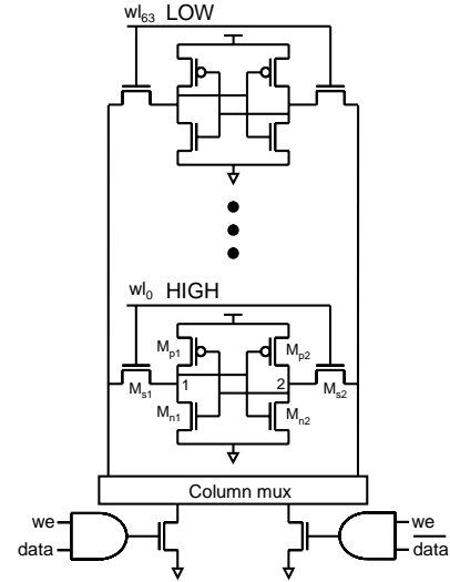
FIGURE 7. 64-bit SRAM column with column mux and write drivers. V_t variation on all devices
